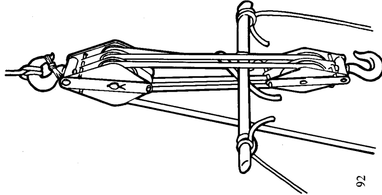
Figure 62. A Three-two Tackle with Anti-twister Fitted
