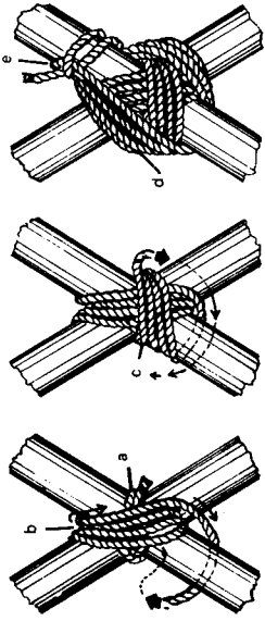
Figure 16. Diagonal Lashing
