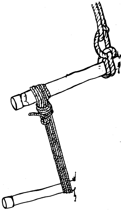
Figure 57. A 1 to 1 Picket Holdfast
