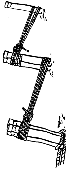
Figure 59. A 3, 2, 1 Picket Holdfast
