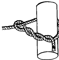
Figure 7. Round Turn and Two Half Hitches
