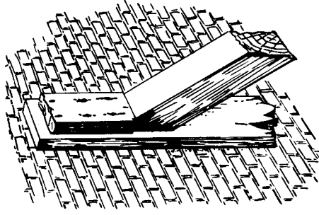
Figure 70. Head of a Raking Shore
