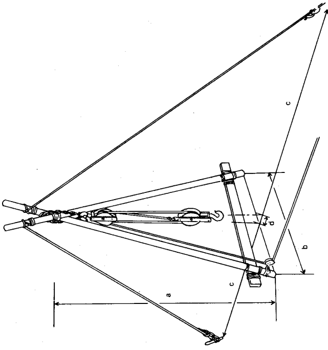
Figure 64. Sheer Legs
