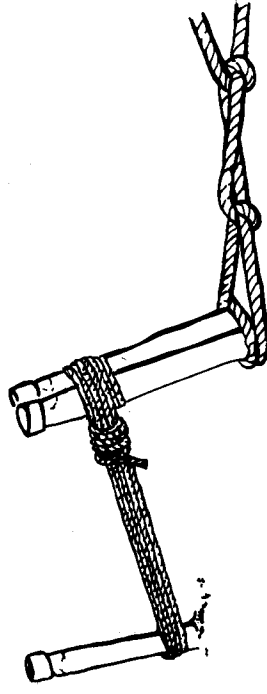
Figure 58. A 2 to 1 Picket Holdfast
