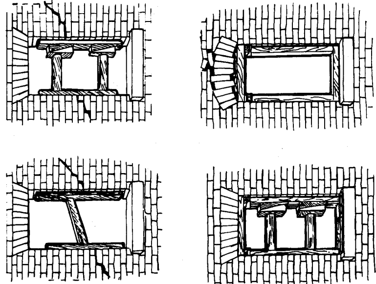
Figure 74. Strutting a Window Opening
