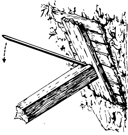
Figure 69. Footing a Raking Shore in soft ground
