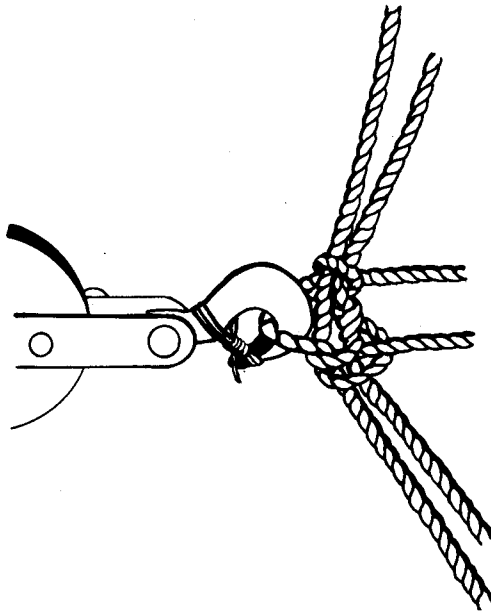
Figure 53 (c). Method of Securing Snatch Lock to Chair Knot
